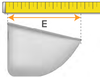
Measure the bucket profile projection "E"
