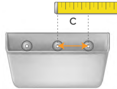
Measure the bucket hole centres "C"
